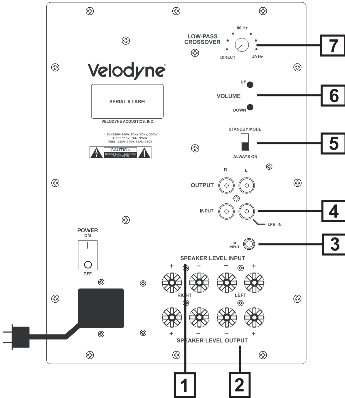
Figure 2. EQ-Max8, EQ-Max10 and EQ-Max12 Rear Panel Connections.
