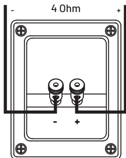
MAD B1-110S connection
